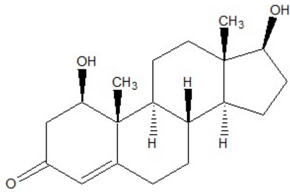
4-Androsten-1beta,17beta-diol-3-one
